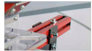
Positioning guides to set a regular distance of the material from the edge and between the eyelets
